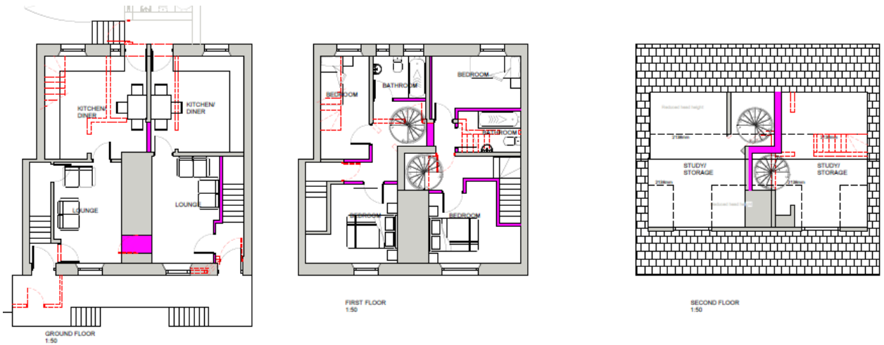
Figure 1.2 Proposed Floor Plans for 74 A King Street
